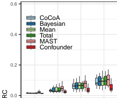
Variance Caused by Disease: 10%
