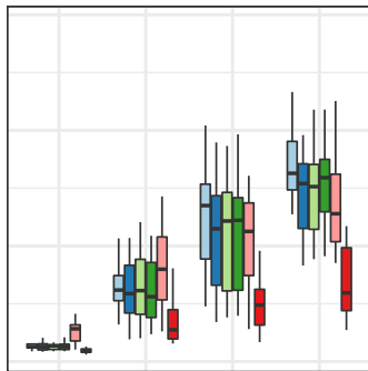
Variance Caused by Disease: 20%
