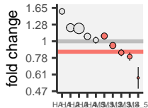
mTconv (7.53e-33)
