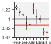
mTreg (2.77e-06)
