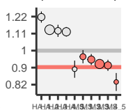
mTreg
